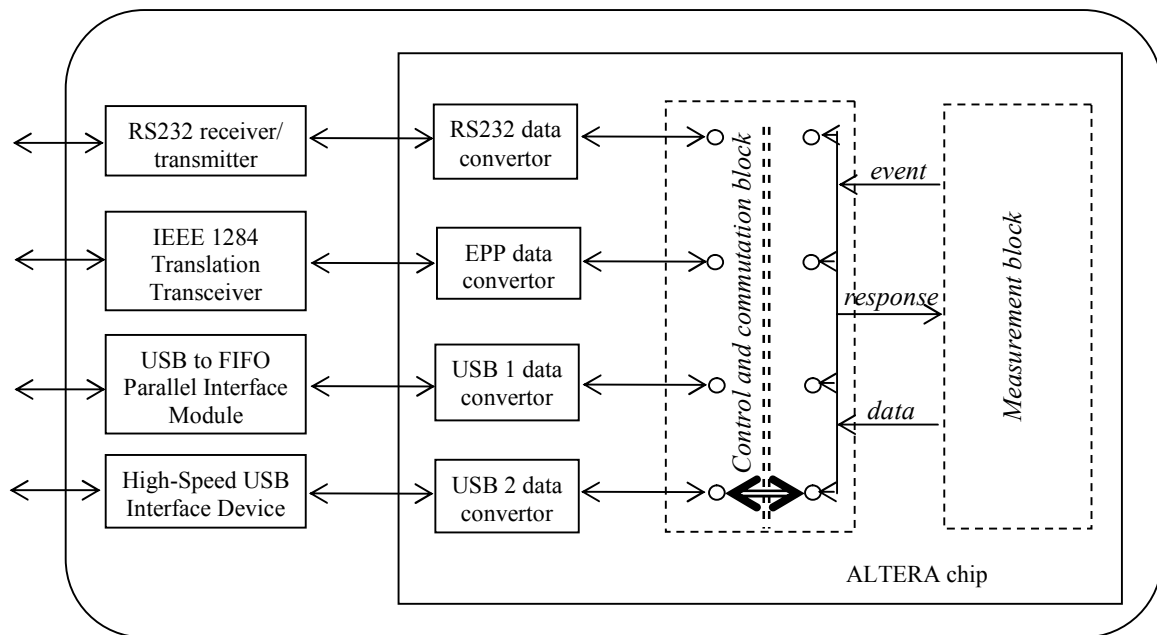
Fig. 3. Schematic block diagram of measurement hardware
