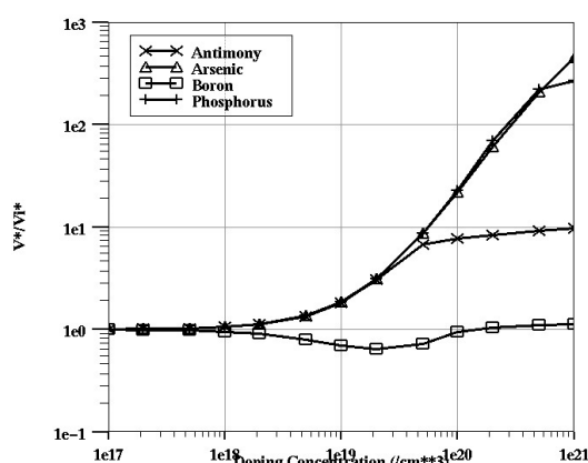
Fig. 1. Simulated V/V i ratio versus doping concentration
