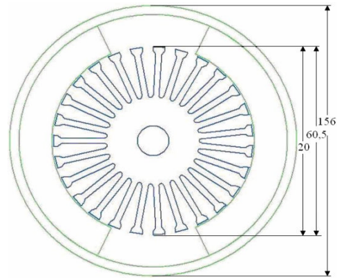
Fig. 4. Iron sheet package view of brushed DC motor with 1.5 kW, 150 rpm permanent magnet
