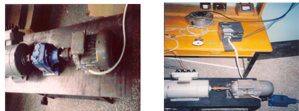
Fig. 1. Experimental mechanisms of 3 phased 1.5 HP motor which is operated with both reductor and inverter
