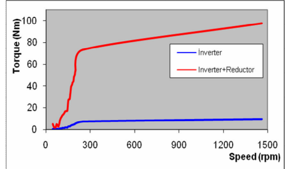
Fig. 2. Torque-speed curves obtained from operating the motor by feeding AC motor with inverter and by combining reductor to its shaft
