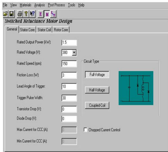
Fig. 7. The window of the program where general information related to 150 rpm, 8/6 pole SR motor is entered.
