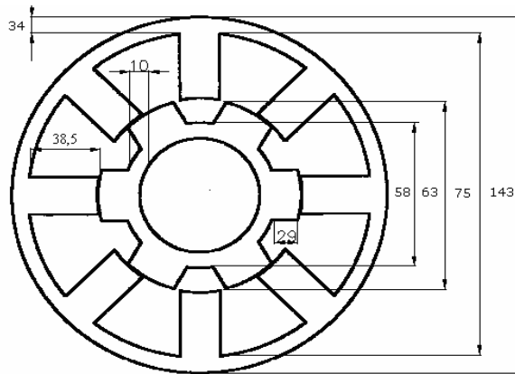
Fig. 8. Iron sheet package view and measurements (mm) of a 1.5 kW, 380 V, 150 rpm, 8/6 pole SR motor.
