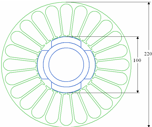
Fig. 6. Iron sheet package view of brushless permanent magnet DC motor
