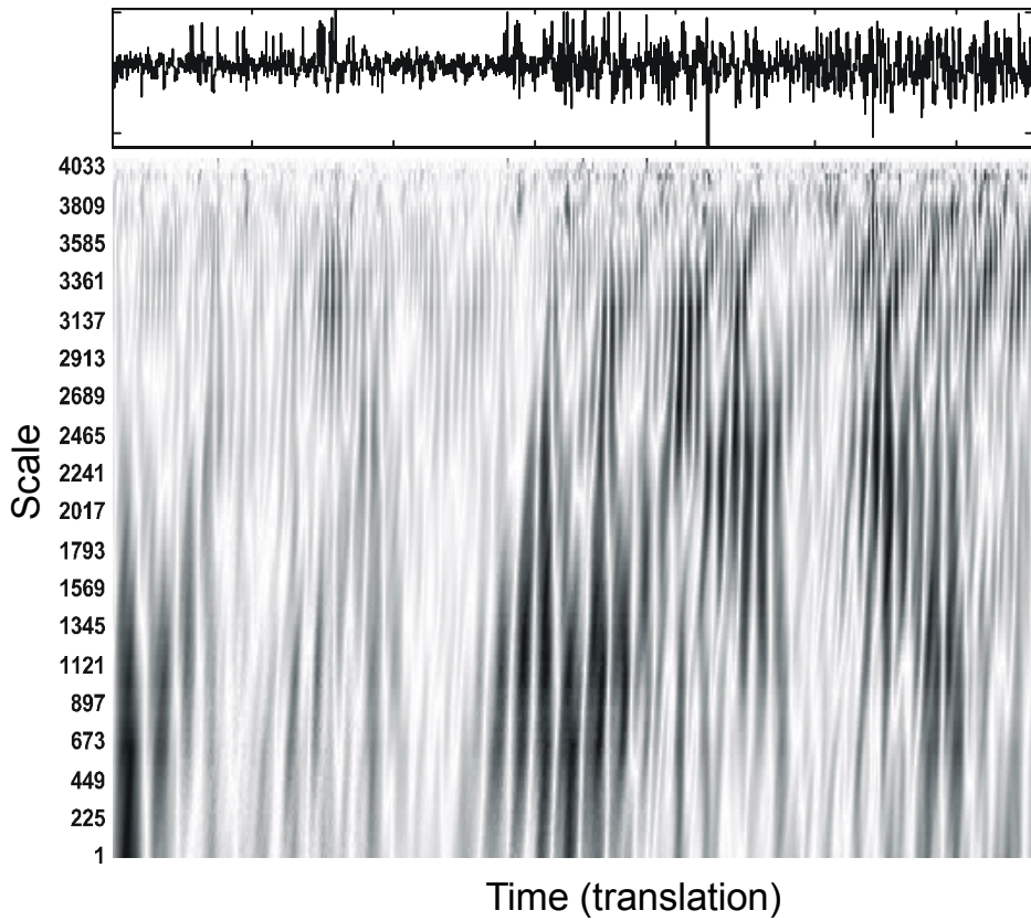
Fig. 5. Scalogram of continuous wavelet transform together with signal being analysed
