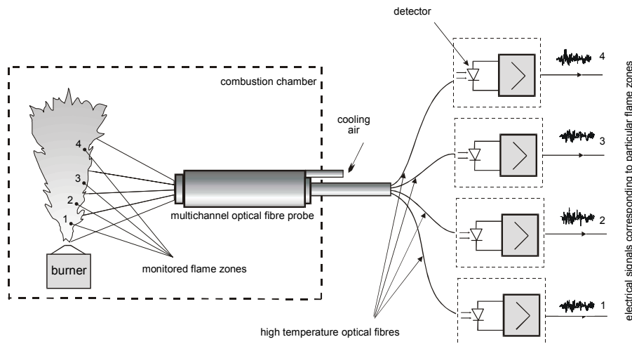
Fig. 2. Block diagram of flame monitoring system
