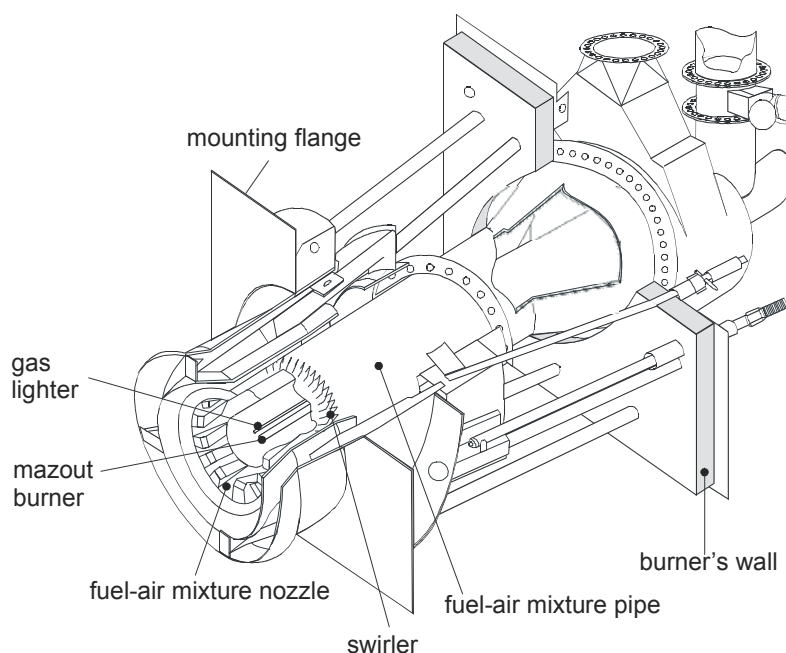
Fig. 1. Pulverised-coal burner with location of mazout burner
