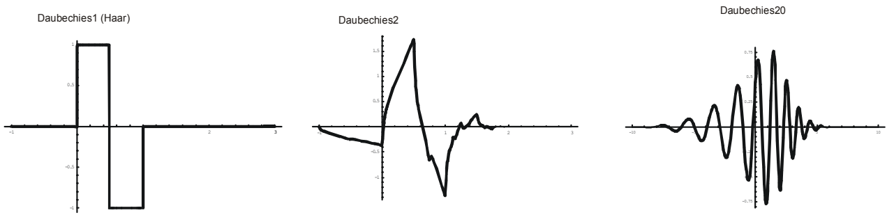
Fig. 3. Daubechies wavelets of various orders
