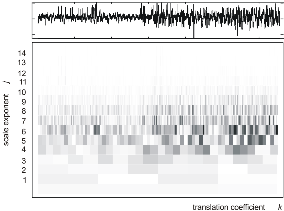
Fig. 5. Scalogram of continuous wavelet transform together with signal being analysed
