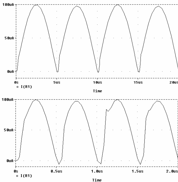
Fig. 9. The output current at 100kHz (above) and 1MHz (bellow)
