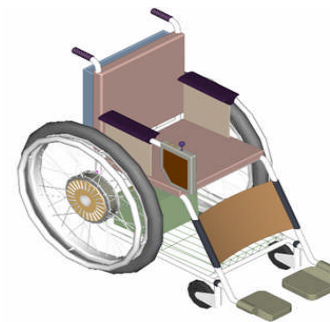
Fig. 17. Perspective views of the integrated design
