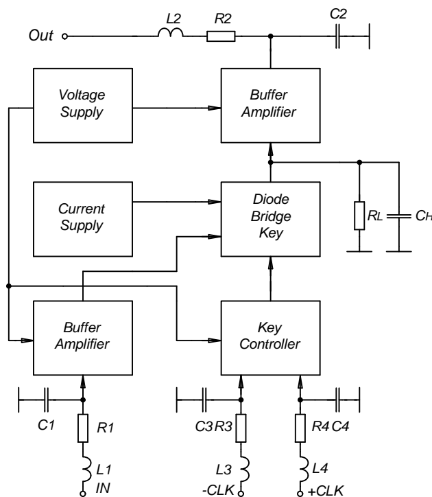
Fig. 1. Simplified track-and-hold circuit
