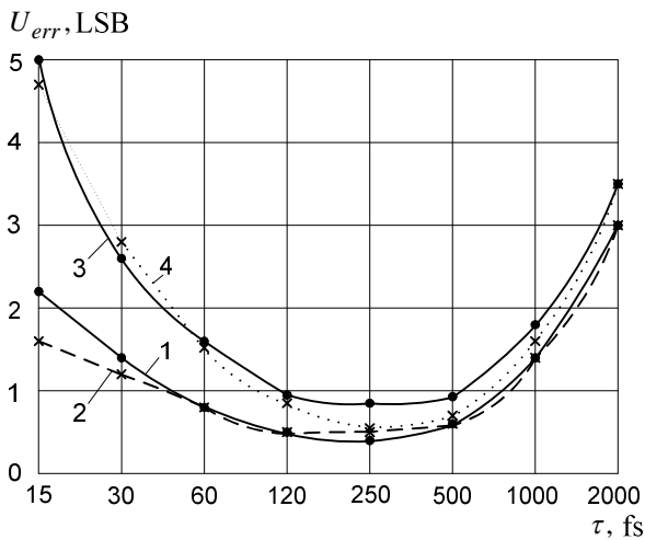
Fig. 4. Dependences of THC errors on \tau . Here curve 1 – 8 bit ADC and L = 0.05 nH, 2 – 8 bit ADC and L = 0.2 nH, 3 – 10 bit ADC and L = 0.05 nH, 4 – 10 bit ADC and L = 0.2 nH
