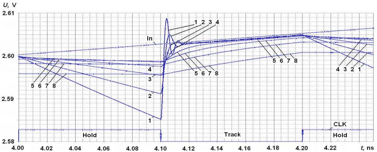
Fig. 3. 10-bit THC time diagrams, when parasitic inductances L = 0.05 nH. Here CLK – 5 GHz clock signal, In – analog input signal, 1 – THC output signal, when \tau = 15 fs, 2 – \tau = 30 fs, 3 – \tau = 60 fs, 4 – \tau = 120 fs, 5 – \tau = 250 fs, 6 – \tau = 0.5 ps, 7 – \tau = 1 ps, 8 – \tau = 2 ps
