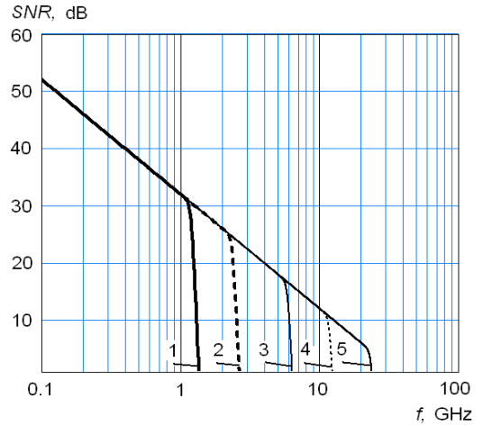
Fig. 5. Dependences of the THC dynamic error in the tracking mode on f when U_0=0.01 V (curve 1); U_0=0.02 V (2); U_0=0.05 V (3); U_0=0.1 V (4); U_0=0.2 V (5)
