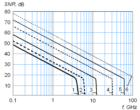
Fig. 6. Dependences of the THC dynamic error in the track mode on f when \tau_E = 3 ps (curve 1); \tau_E = 2 ps (2); \tau_E = 1 ps (3); \tau_E = 0.4 ps (4); \tau_E = 0.2 ps (5); \tau_E = 0.1 ps (6)
