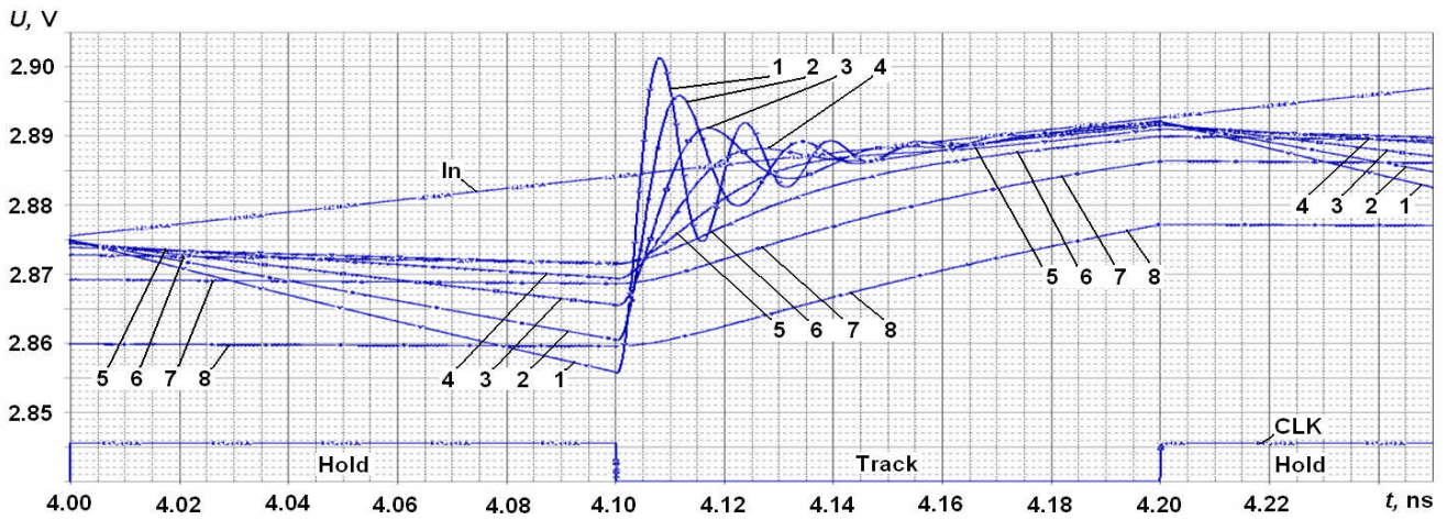
Fig. 2. 8-bit THC time diagrams, when parasitic inductances L = 0.2 nH. Here CLK – 5 GHz clock signal, In – analog input signal, 1 – THC output signal, when \tau = 15 fs, 2 – \tau = 30 fs, 3 – \tau = 60 fs, 4 – \tau = 120 fs, 5 – \tau = 250 fs, 6 – \tau = 0.5 ps, 7 – \tau = 1 ps, 8 – \tau = 2 ps
