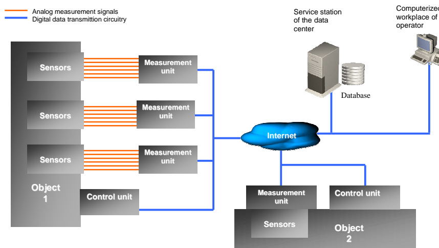
Fig. 1. Block diagram of monitoring system
