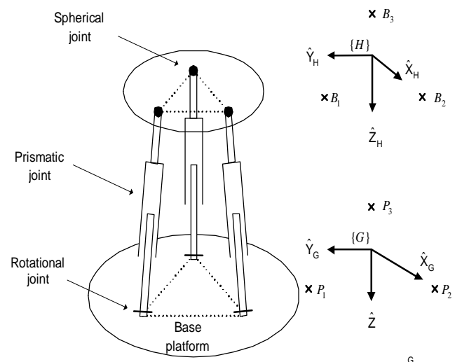
Fig. 1. Schematic representation and coordinate systems of the 3-RPS manipulator
