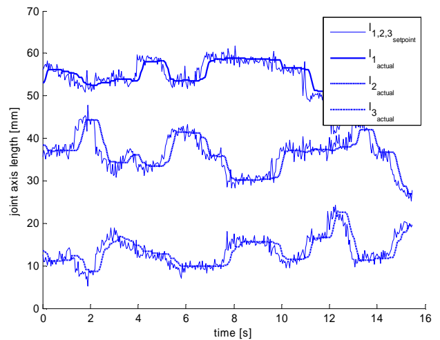
Fig. 3. Actuating lengths of the prismatic joint axes (setpoint and actual values)
