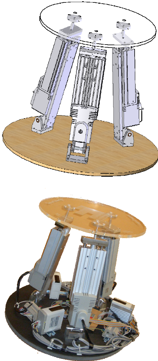
Fig. 2. CAD-model and photograph of the 3-RPS manipulator
