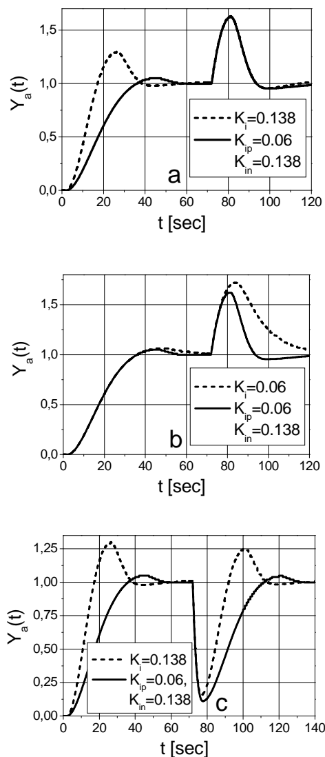
Fig. 4. Unit set point step response followed by the positive (a, b) and negative (c) unit load disturbances of the control system with the plant G_I(s) based on I (dashed line) and aI (solid line) controllers. The I controller is adjusted to dynamics of the plant associated with b = 2 (a, c) and b = 7 (b)
