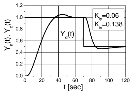
Fig. 3. The unit set point step response followed by the Y_d drop of the control system with the plant G_I(s) based on the aI controller
