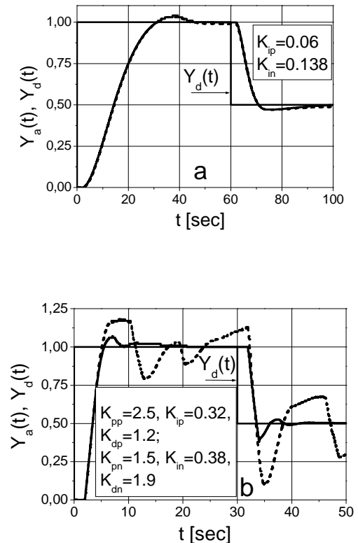
Fig. 5. The unit set point step response followed by the Y_d drop of the control system with the plant G_I(s) based on the aI (a) and aPID (b) controllers affected by the sinus noise (dashed line) and not affected by noise (solid line) (the amplitude of noise 0.05, frequency 50 Hz; the parameters of the aPID controller with the index p act at positive values of e(t) and with the index n – at negative values)
