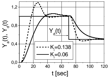
Fig. 2. The unit set point step response followed by the Y_d drop of the control system with the plant G_I(s) based on the I controller adjusted to dynamics of the plant associated with b = 2 (dashed line) and b = 7 (solid line)
