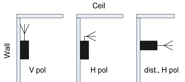
Fig. 2. AP setup for corridor measurements
