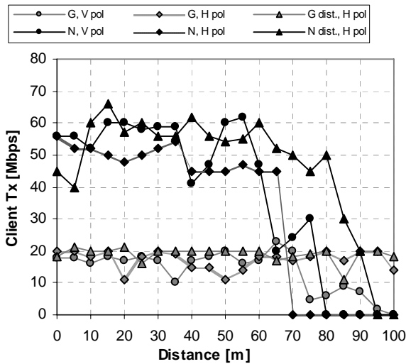
Fig. 4. Client transmitting distance and bandwidth estimation to AP
