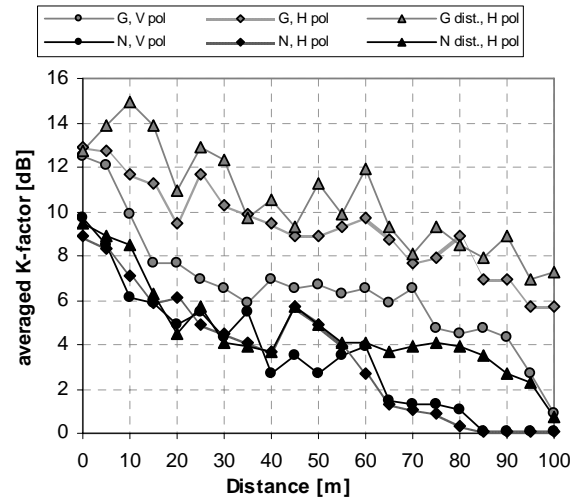
Fig. 6. Average Ricean K-factor vs. distance and polarisation for 802.11g and 802.11n devices in long corridor
