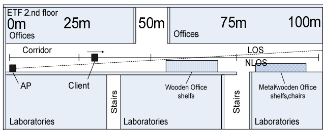
Fig. 1. Overview of measurement environment
