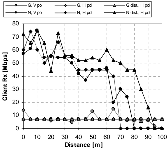
Fig. 5. Client receiving distance and bandwidth estimation to AP
