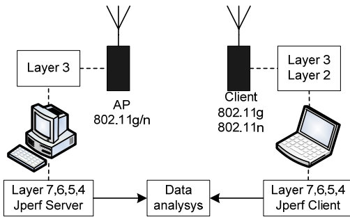
Fig. 3. Measurement system setup
