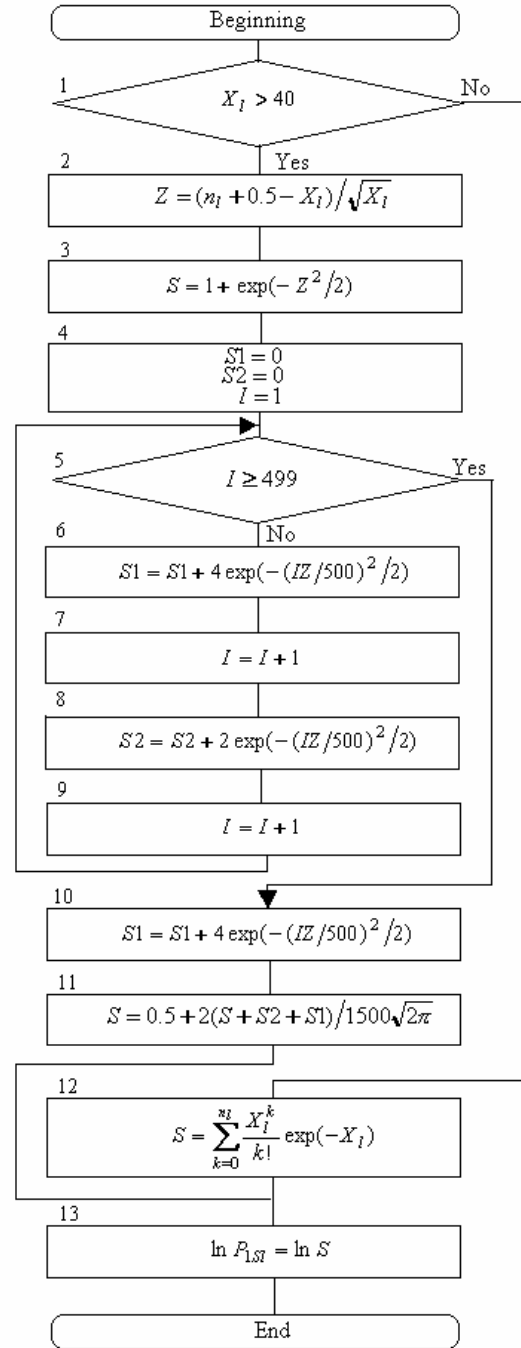
Fig. 2. The flowchart of algorithm of function LPS (subroutine)
