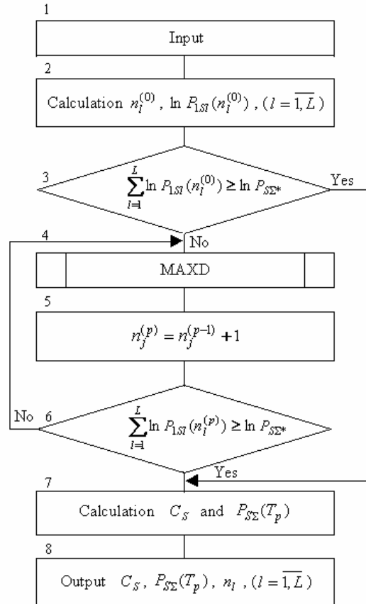
Fig. 1. The flowchart of algorithm of the program of calculation of stocks a component
