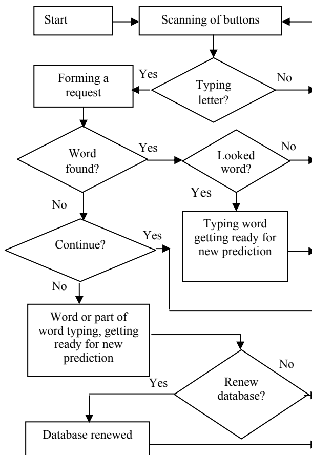
Fig. 3. Prediction algorithm
