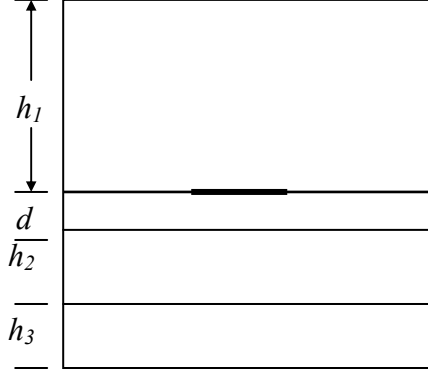
(c) Three layer microstrip line
