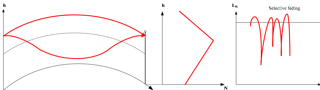
Fig. 1. Multipath fading due to surface inversion layer
