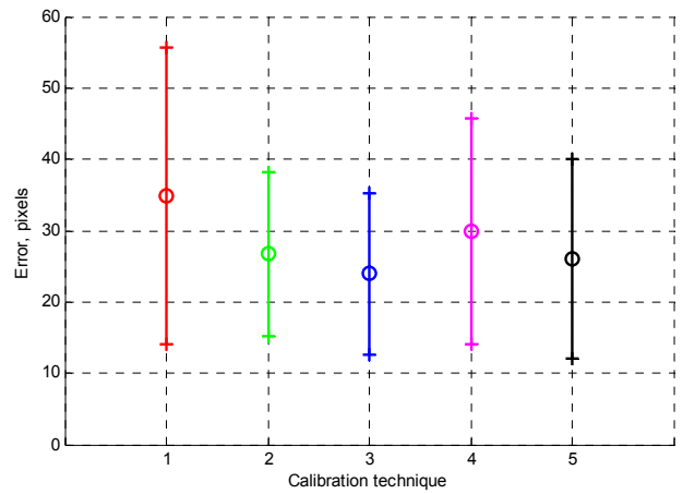
Fig. 7. Averaged mapping errors of different calibration techniques. “o” – mean value, “+”- standard deviation
