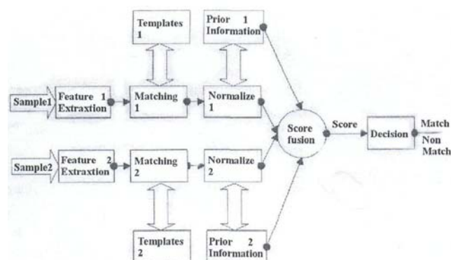
Fig. 1. A schematic for score level fusion
