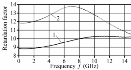
Fig. 8. Frequency dependences of retardation factors: 1 – of the symmetric meander system; 2 – of the system with shifted meander electrodes
