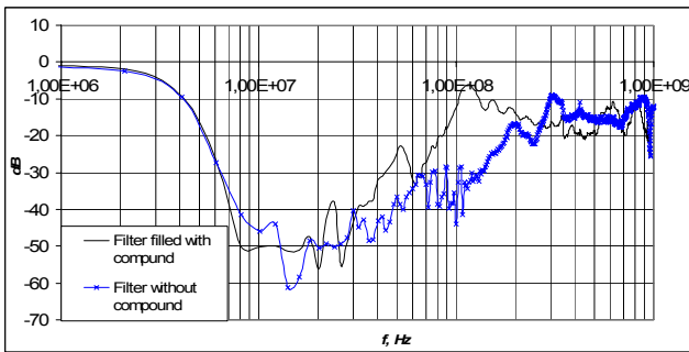
Fig. 6. Filter filled with compound and filter without compound
