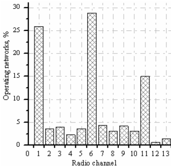
Fig. 3. The frequency channels used in discovered infrastructure and ad-hoc networks
