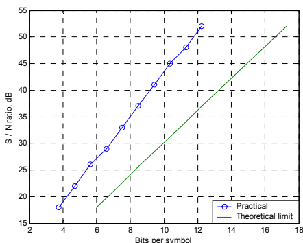
Fig. 3. Practical bit-per-symbol values and theoretical limit
