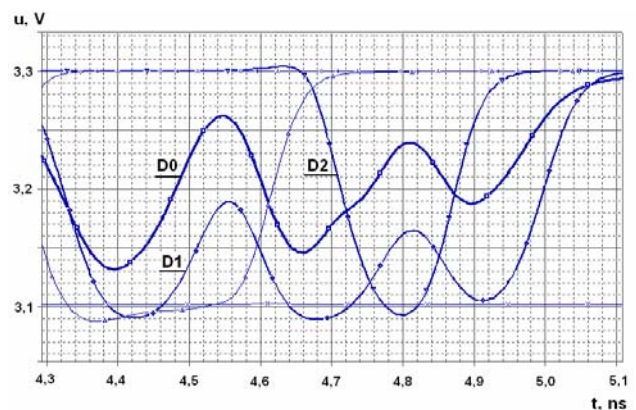
Fig. 6. ADC output signals at the 40 MHz input frequency
