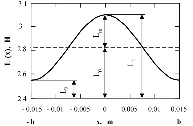
Fig. 1. Dependence of inductivity for 100 V direct (constant) power supply voltage
