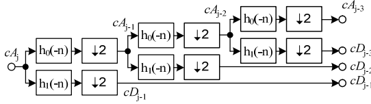
Fig. 4. The set of three - leveled analysis filters
