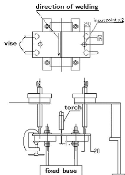
Fig. 1. Set of specimens (mm)
