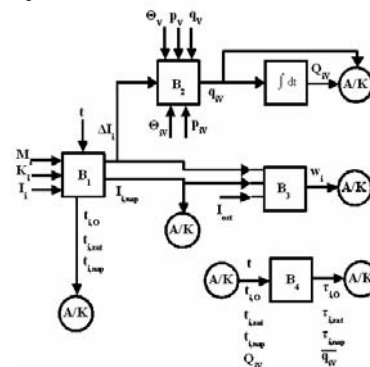
Fig. 4. Block diagram
