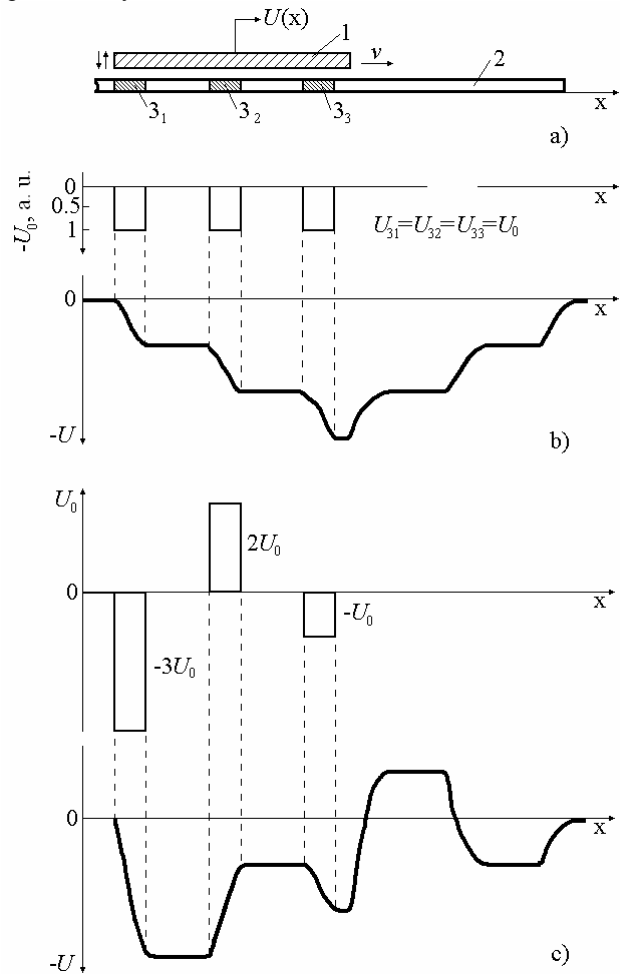
Fig. 5. Constructed experimental model of some defective areas (a) and measured surface electric potential when potential of defective areas are equal and same sign (b) or different values and signs (c). Potential of defective area is far greater than measured.
