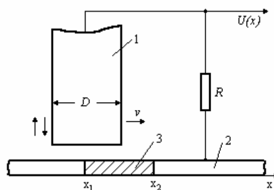
Fig. 1. Model of vibrating electrode (1) and surface of sample under investigation (2). 3 – defective area which diameter is x_2 - x_1 = D , v – speed of electrode shift (scanning)
