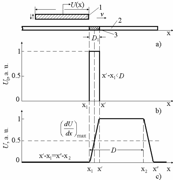
Fig. 4. Accepted model of defective area (a), constructed surface electric potential (b) and measured electric potential (c). Defective area's size is less the diameter of vibrating probe and U_0 \gg U .
