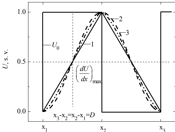
Fig. 2. Accepted character of surface potential U_0 , which characterizes the informative area and the measured potential, when the electrode's tip and informative area are such: square-strip (1), circle-strip (2), circle-circle (3).
