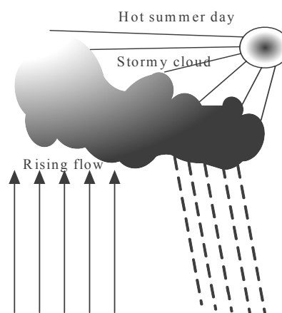
Fig. 2. Convective precipitation
