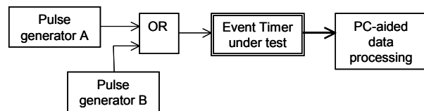
Fig.1. Test circuits for linearity evaluation
