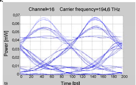
Fig. 8. Output eye diagrams: a) channel number 10, b) channel number 16
