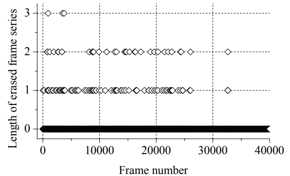
Fig. 5. Experimentally collected frame erasure trace
