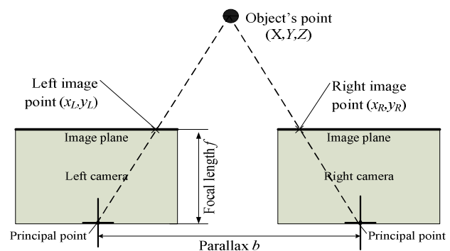
Fig. 1. Illustration of the stereo geometry
