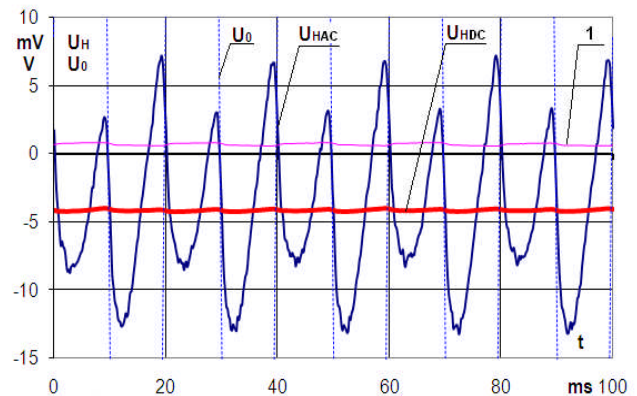
Fig. 1. Hall voltage U_H value (AC and DC components – U_{HAC} , U_{HDC} ) versus time for healthy feeder under symmetrical 3-phase load (50 A) when zero sequence voltage ( U_0=100V ) is applied ( I_{load}=0 )
