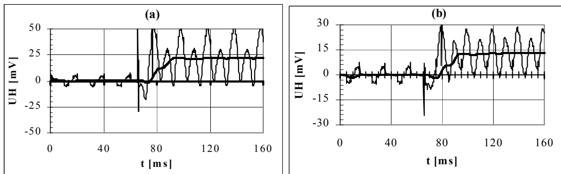
Fig. 6. Hall output voltage in a case of one phase metallic and resistive ground faults in the 6kV feeder of a strip mine operating with isolated neutral point: a) metallic short-circuit ( U_o=100V , 3I_o=2.8A ); b) metallic short-circuit ( U_o=67V , 3I_o=1.8A )
