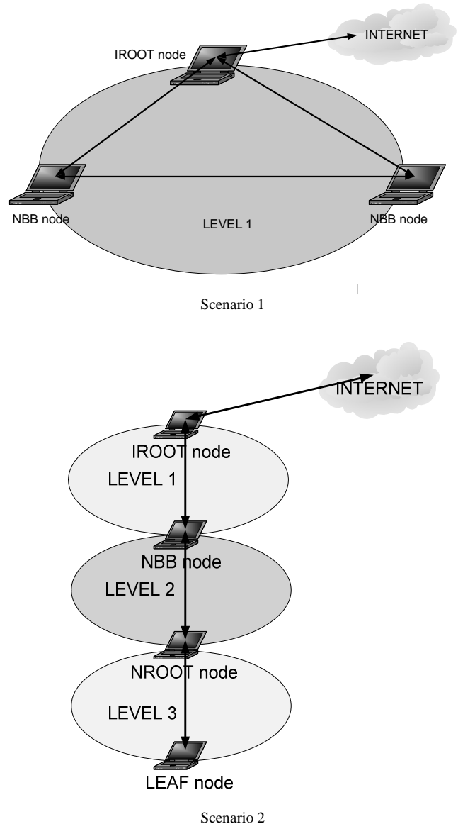
Fig. 2. Scenarios 1 and 2, used to evaluate the PANDORA protocol
