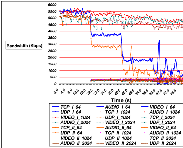
Fig. 3. Bandwidth used by different traffic flows without applying any queuing discipline using 64, 1024 and 2024-bytes packets
