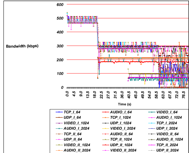
Fig. 6. Bandwidth used for the different trafficflows with DSMARK qdisc and 64, 1024, 2024-bytes packets
