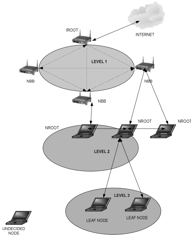
Fig. 1. PANDORA Protocol
