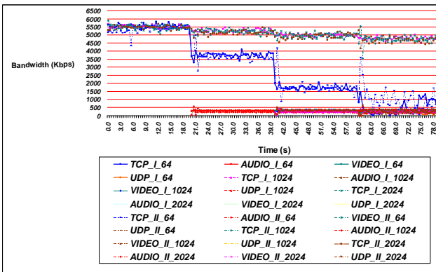
Fig. 4. Bandwidth used by different traffic flows with PRIO qdisc and 64, 1024 and 2024-bytes packets
