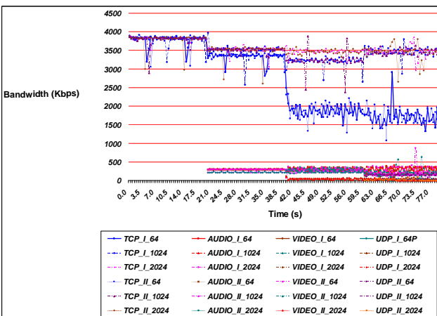
Fig. 5. Bandwidth used for the different traffic flows with HTB qdisc prioritizing the audio, and 64, 1024 and 2024-bytes packets
