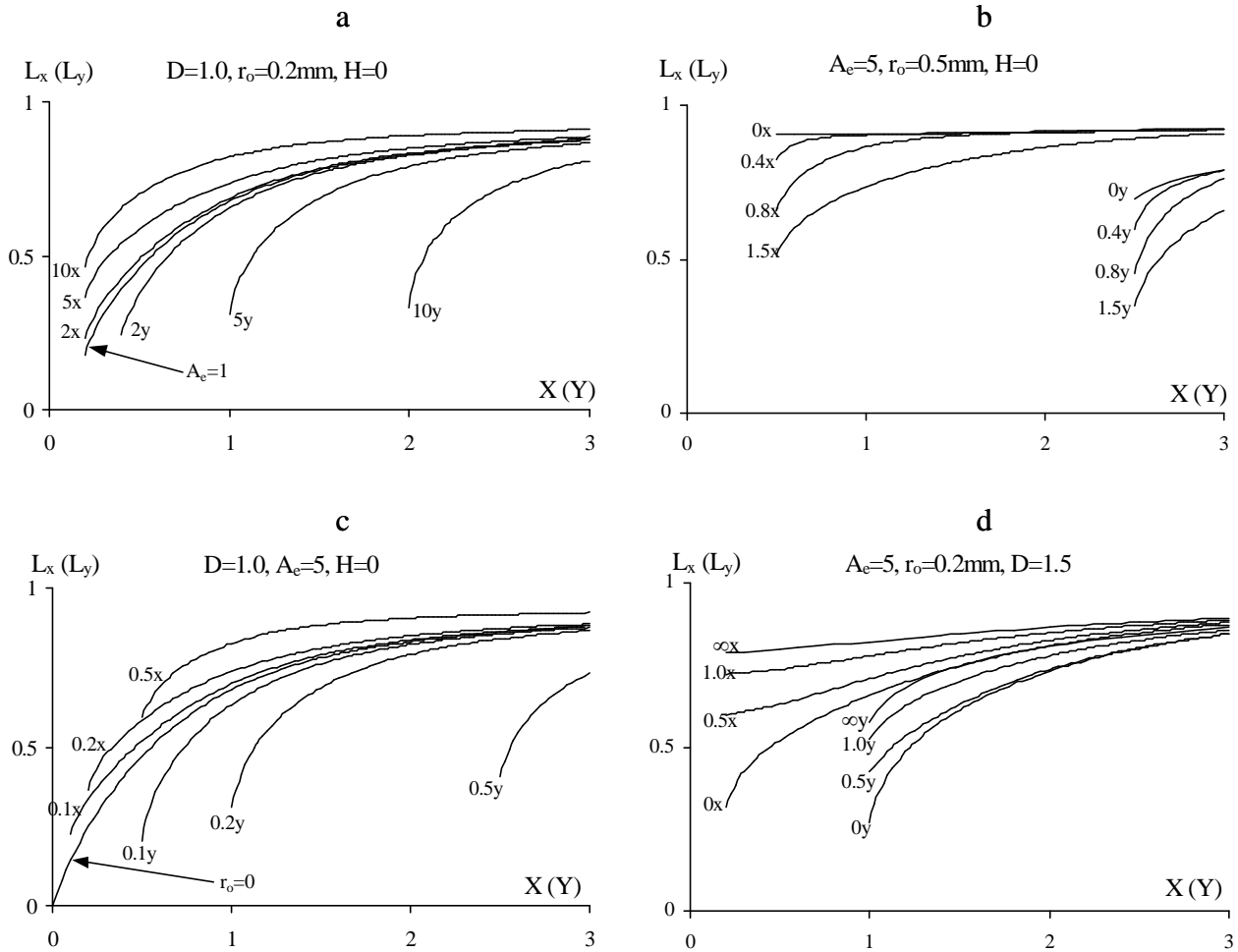
Fig. 1. Dependence of L_x and L_y on parameters of three-dimensional medium and a distance of recording site from a current electrode center ( X or Y ). “ x ” next to curves refers to the dependence of L_x on X , and “ y ” – the dependence of L_y on Y . In all cases \lambda_x = 1.0 mm. a: for all curves D = 1.0 , r_o = 0.2 mm, H = 0 , and numbers -1, 2, 5, 10 – are values of electrotonic anisotropy; b: for all curves A_e = 5 , r_o = 0.5 mm, H = 0 ; the numbers -0, 0.4, 0.8, 1.5 – are the normalized thickness ( D ) of the medium; c: for all curves D = 1.0 , A_e = 5 , H = 0 ; the numbers 0.1, 0.2, 0.5 – are radii of the current electrode in mm; d: for all curves D = 1.5 , A_e = 5 , r_o = 0.2 mm; the numbers 0, 0.5, 1.0 – are normalized altitudes ( H ) of cylinder-shaped current electrode; \infty - refers to case when H \rightarrow \infty and D \rightarrow \infty .
