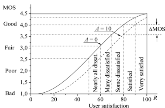
Fig. 2. Application of E-model for user satisfaction estimation
