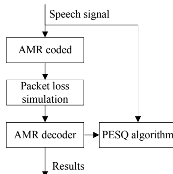
Fig. 3. Simulation scheme
