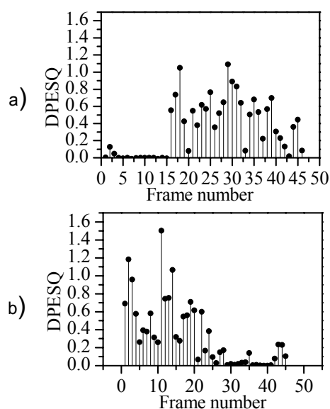
Fig. 4. DPESQ as function of position of lost frame: a) word “mama”, b) word “namas”
