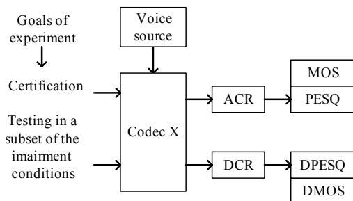
Fig. 1. Voice quality evaluation methods
