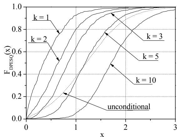
Fig 5. Empirical conditional cumulative distribution functions of quality degradation
