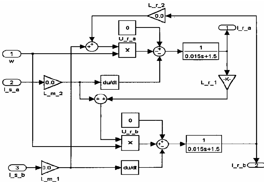
Fig. 1. Block diagram of the model of squirrel-cage rotor of induction motor
