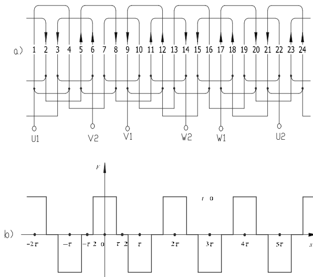
Fig. 2. Connection scheme of eight-pole concentrated three-phase windings (a) and the distribution of its rotating magnetomotive force in time moment t = 0 (b)
