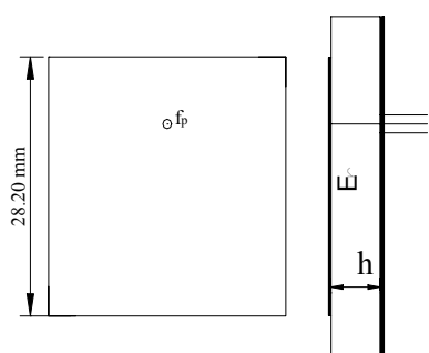
Fig. 1. A microstrip Patch Antenna
