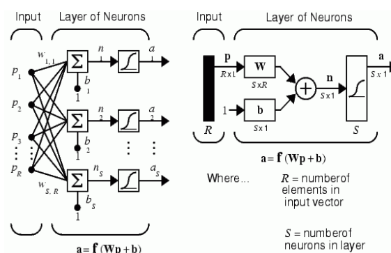
Fig. 2. Feed forward Network
