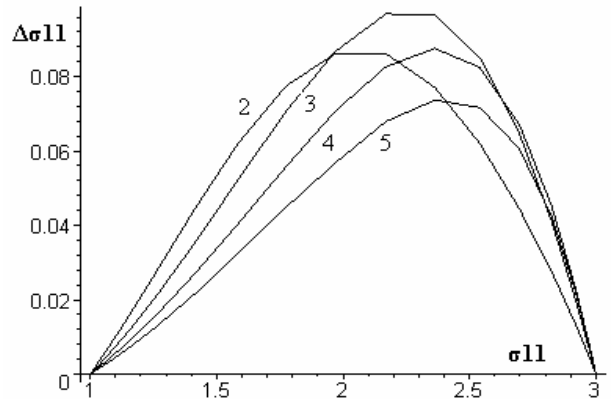
Fig. 5. Errors \tilde{\sigma}_{ij} - \sigma_{ij} of the tensor components. The numbers in the graph show ratio a/b between the side lengths of rectangle.
