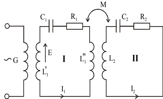
Fig. 4. The equivalent circuit of HM
