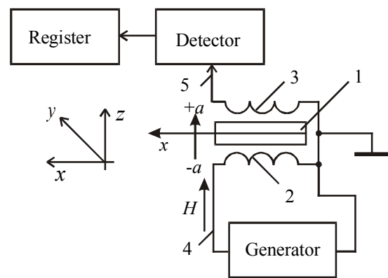
Fig. 1. The experimental device of Helicon Maser
