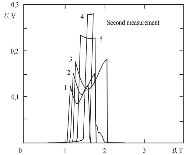
Fig. 3. The resonance curves of the HM for various frequencies of excitation: 1 – 19,3 MHz; 2 – 19,5 MHz; 3 – 19,7 MHz; 4 – 20 MHz (generation frequency); 5 – 20,5 MHz; U – the signal of pickup coil in Volts; B – magnetic field induction in Tesla
