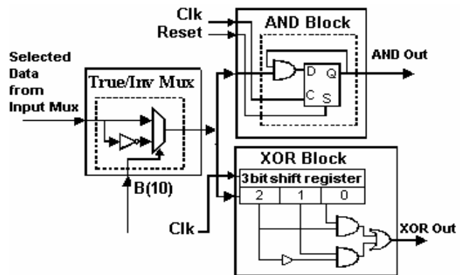
Fig. 4. Structure of Single Bit Processor with AND and XOR blocks
