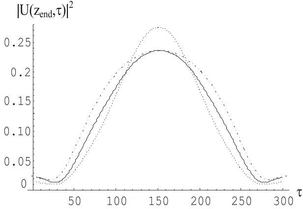
Fig. 2. Pulse shape at the end of the optical fiber in case of propagation of Gaussian pulse: z=23 L_D , ( N^2 \ll 1 ), SIR =10 dB, \varphi=\pi : dotted curve – interference appears at z_{ap}=3L_D ; solid curve – z_{ap}=10L_D ; dash-dotted curve – z_{ap}=20L_D
