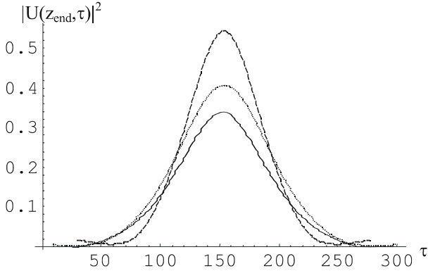
Fig. 3. Pulse shape at the end of the optical fiber in case of propagation of Gaussian pulse: z=23 L_D ( N^2 \approx 1 ), SIR =10 dB, \varphi = \pi : solid curve – interference appears at z_{ap}=3L_D ; dotted curve – z_{ap}=10L_D ; dashed curve – z_{ap}=20L_D
