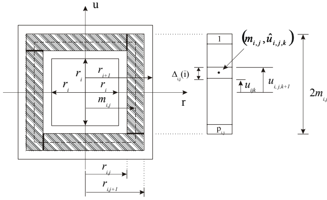
Fig. 1. Two-dimensional space partitioning
