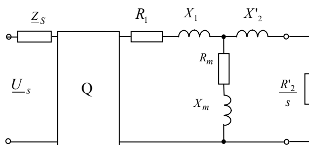
Fig. 1. Per-phase equivalent circuit of cage induction motor with the supply cable and the inner complex impedance of the power-supply source Z_s ; U_s is the complex voltage of power-supply source; Q is the four-pole; R_1 , X_1 , R_m , X_m , X'_2 , R'_2 is the L -type equivalent circuit parameters of a cage induction motor; s is the slip
