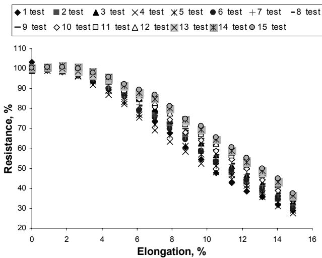
Fig. 7. Resistance changes of the IV sample versus its extension (pressure of 2.5 atmospheres)
