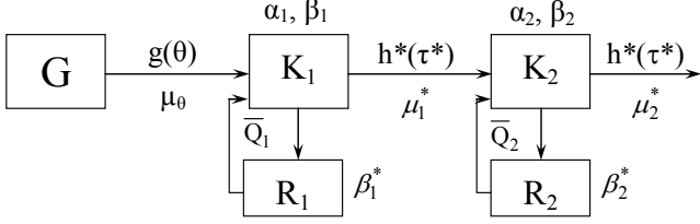
Fig. 3. The modified two-stage continuous control
