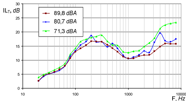
Fig. 9. The dependence IL_T on the environment noise SPL
