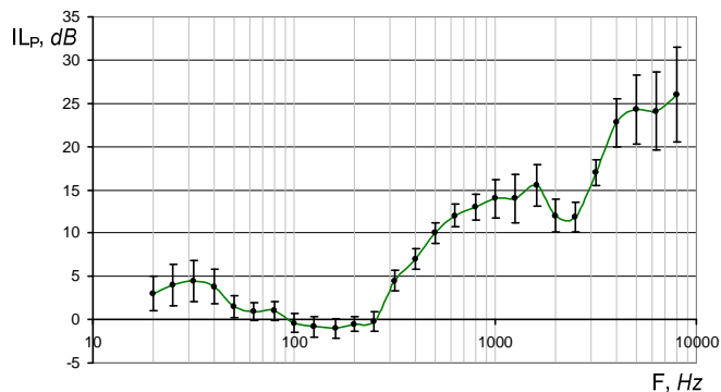
Fig. 10. The passive insertion loss of industrial production head sets
