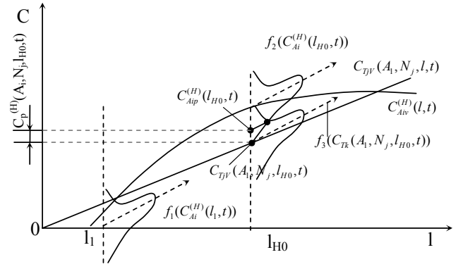
Fig. 10. The finding of the value C_p^{(H)}(A_i, N_j, l_{H0}, t)
