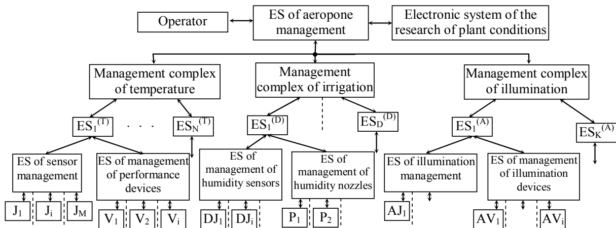
Fig. 6. ES of aeropone management ( E_i^{(T)} , ES_i^{(D)} and ES_i^{(A)} , – ES of management of i -th temperature, humidity and illumination components; J_i , V_i – temperature sensors and performance devices; DJ_i or P_i – humidity sensor and nozzle)
